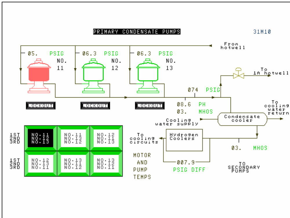
Figure 4. Honeywell TDC3000 Screen for Condensate Control
