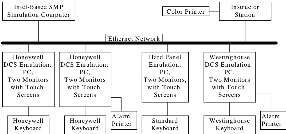
Figure 1. Configuration of Bergen Compact Simulator
